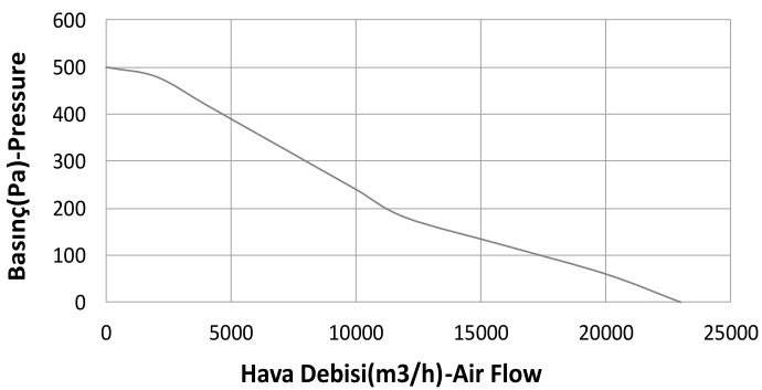
G800 - 2.2 kw
