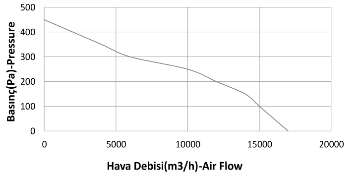
G800 - 3 kw
