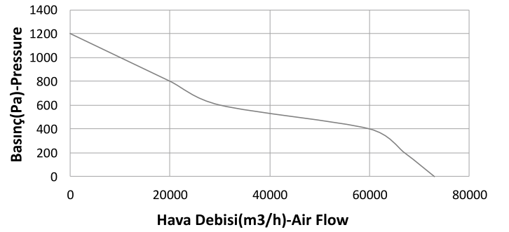
G1120 - 30 kw
