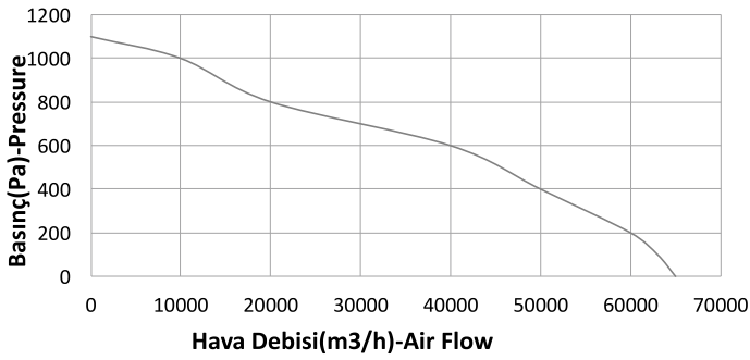
G1120 - 22 kw
