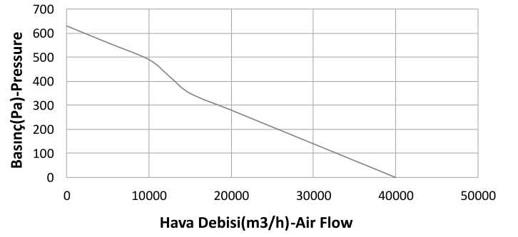
G1000 - 7.5 kw
