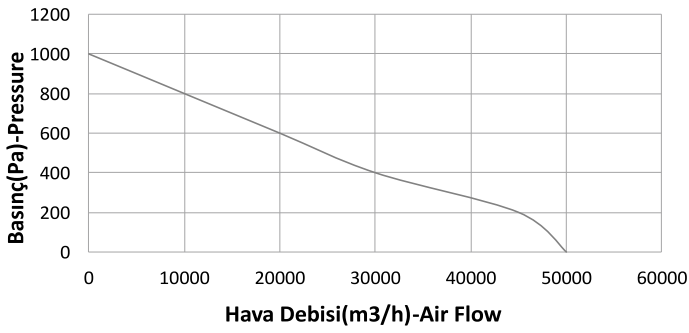
G1000 - 15 kw
