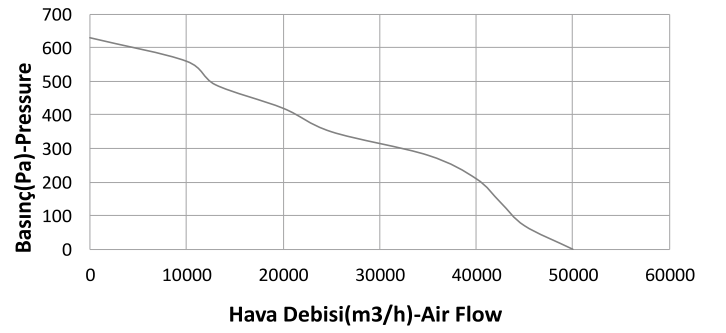
G1000 - 18.5 kw
